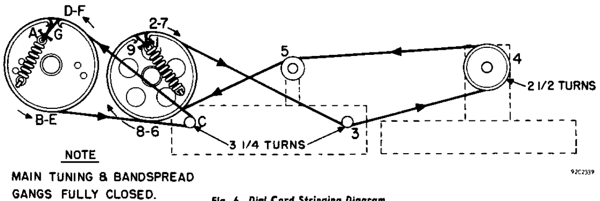
Fig. 6. Dial Cord Stringing Diagram
