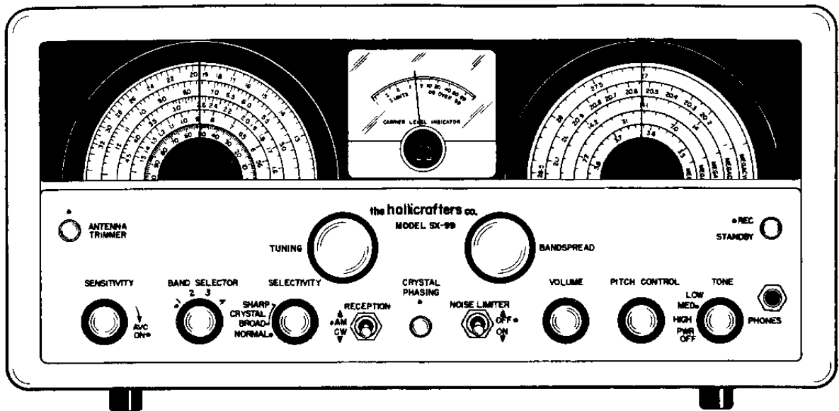
Fig. 4. Operating Controls
