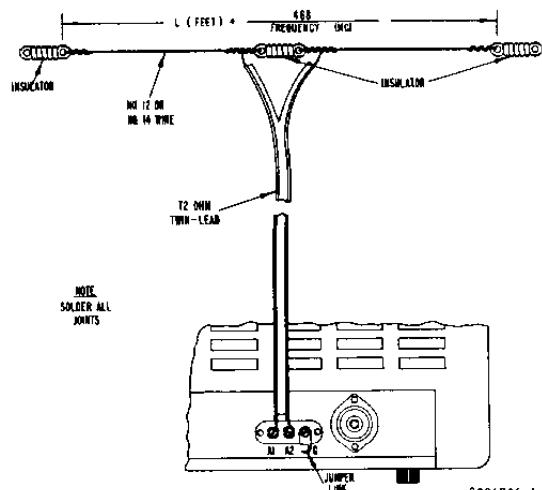
Fig. 3. Doublet Antenna Using Twin-Lead Lead-In
